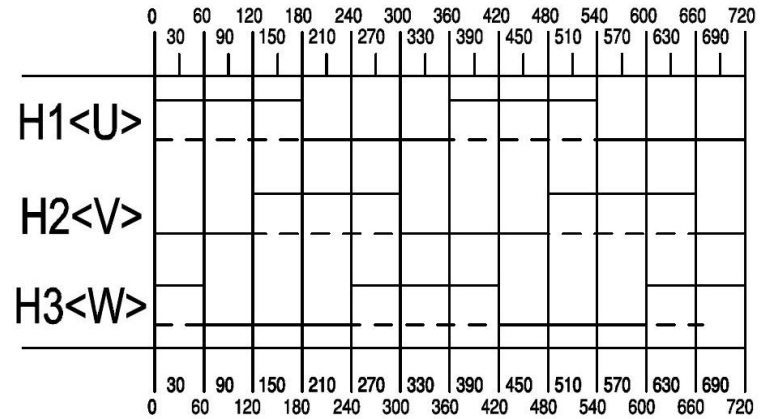
Electrical Angle
