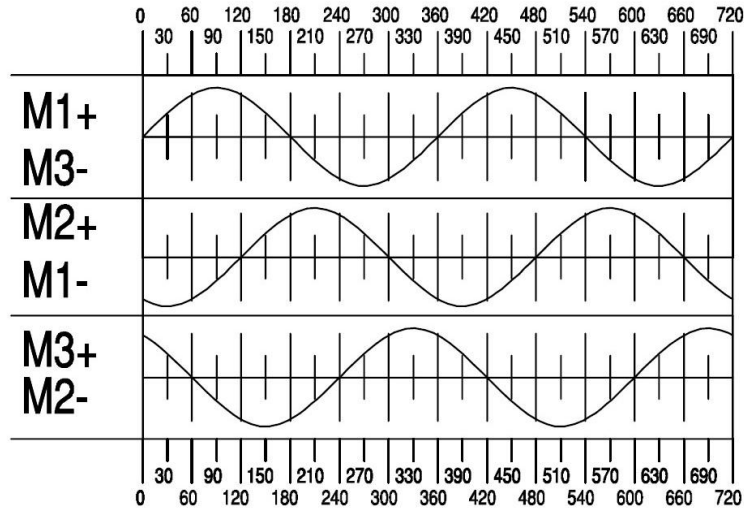
Electrical Angle
